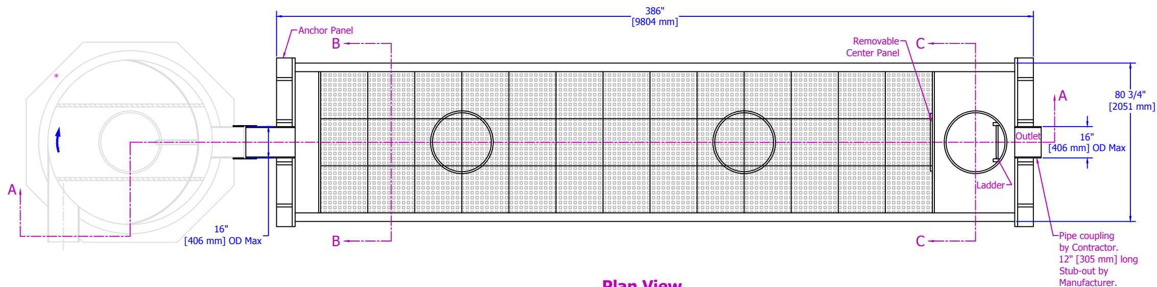
Plan View
