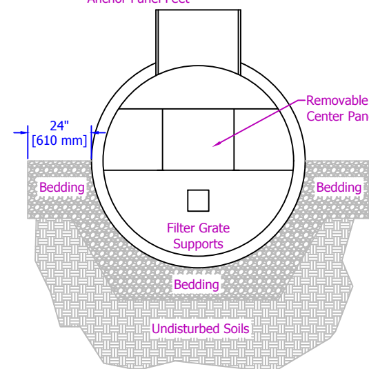
Section C-C
